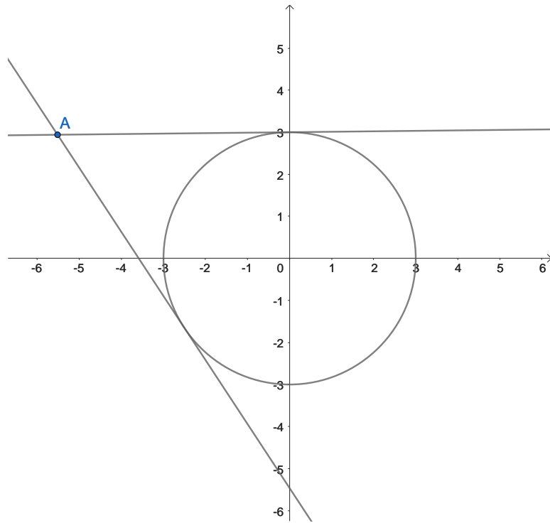
FIGURE 1. A Geogebra picture
